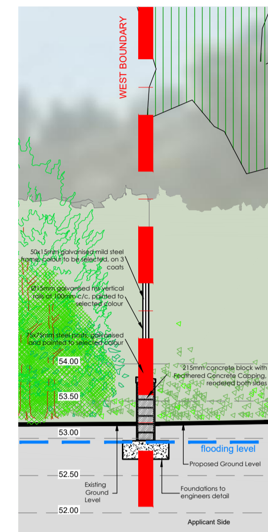
FENCE DETAIL C1 (Scale 1:50)
