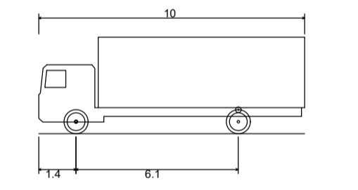
FTA Design 13/18 Tonne Rigid Vehicle (2016)
