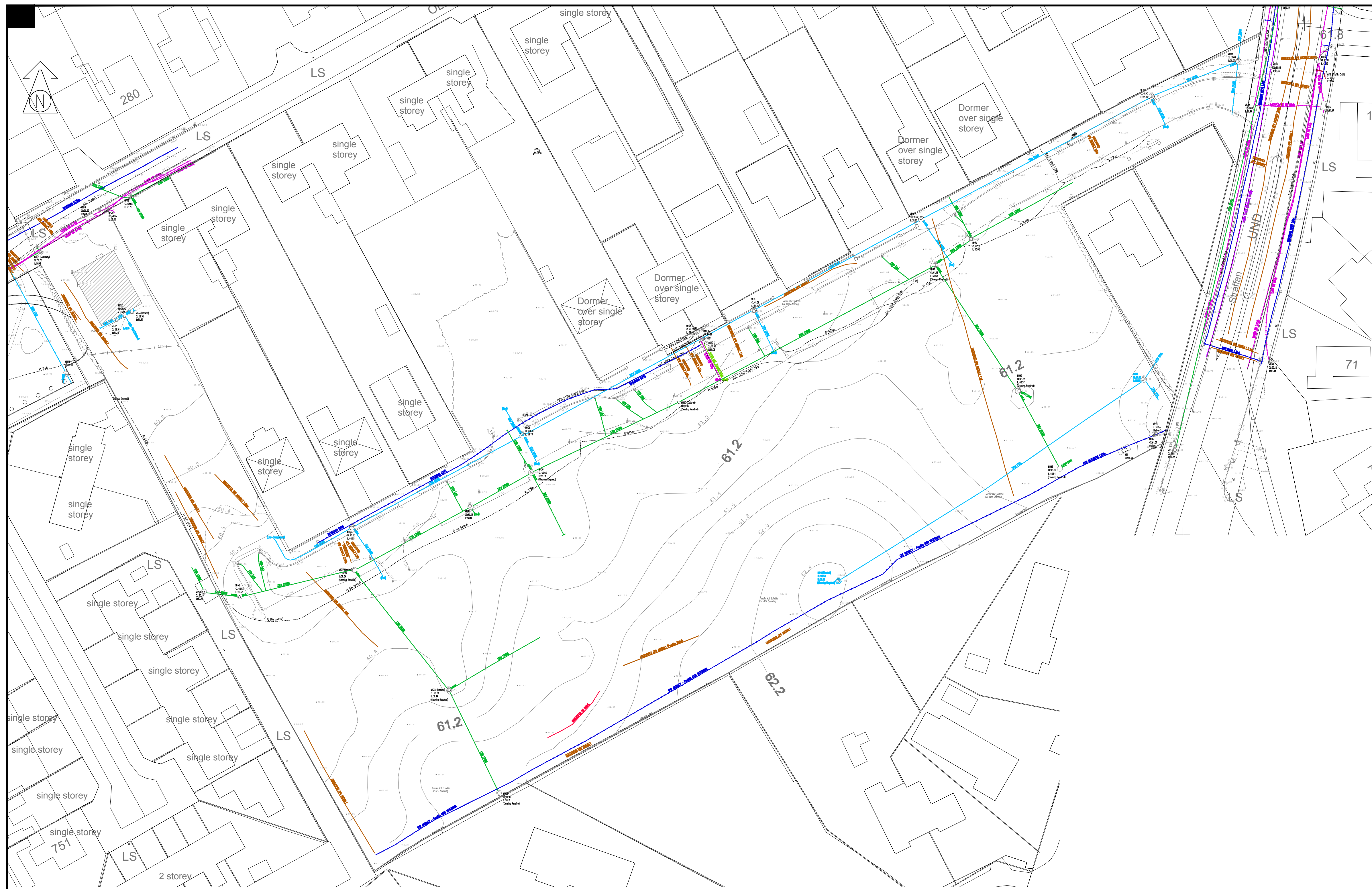
EXISTING SITE & SERVICES LAYOUT SCALE 1:500
