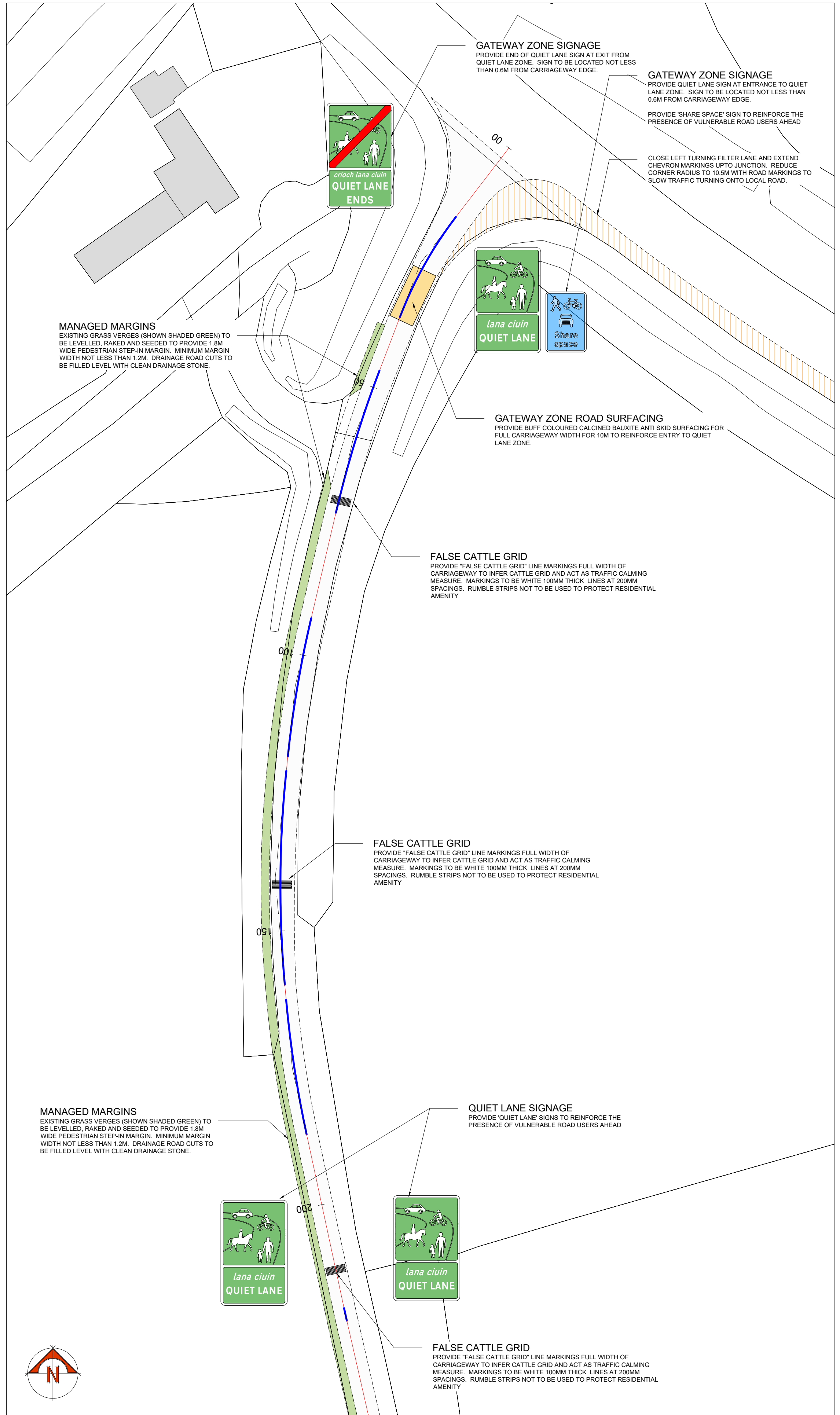
DETAILED LAYOUT 01 SCALE 1:500
