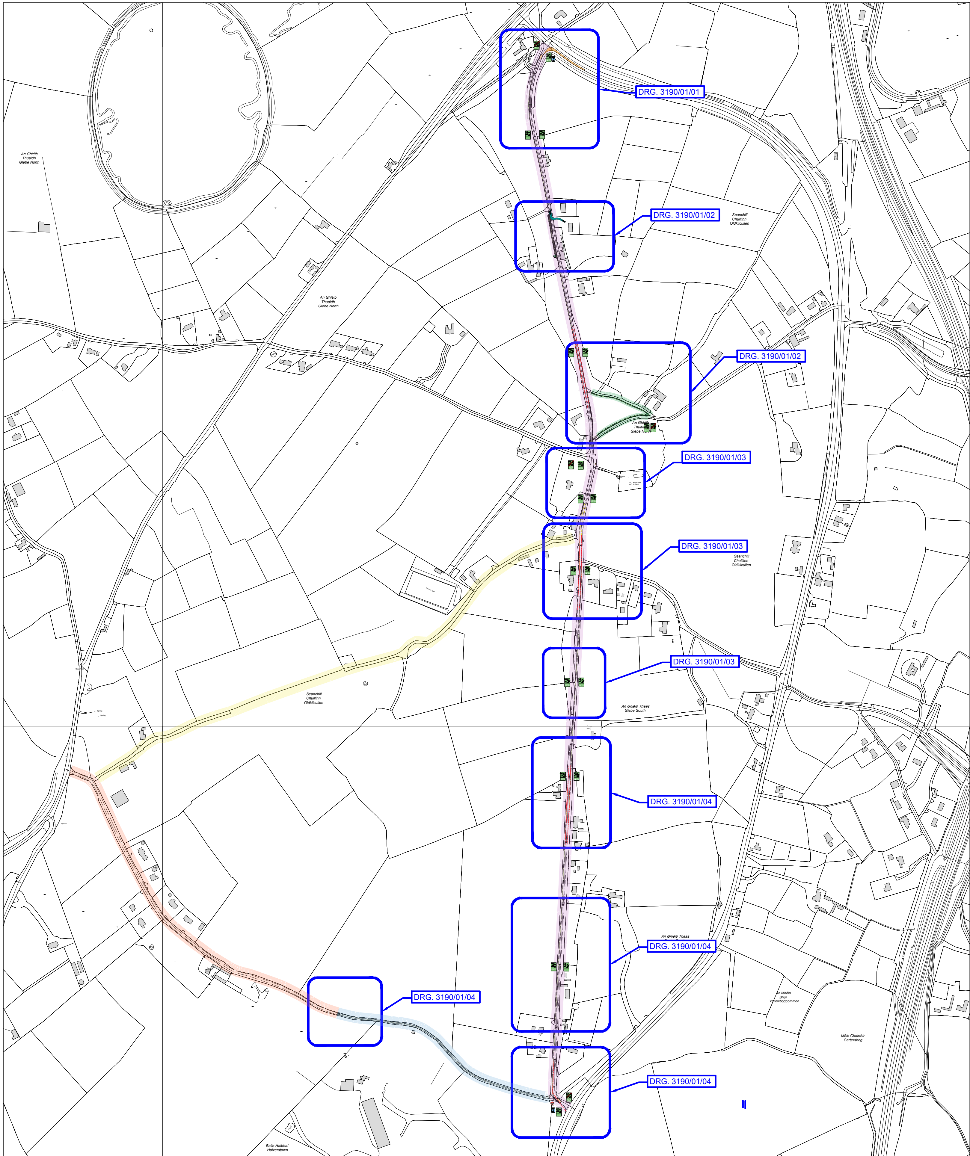
SITE LAYOUT - GENERAL ARRANGEMENT + KEY PLAN SCALE 1:5000
