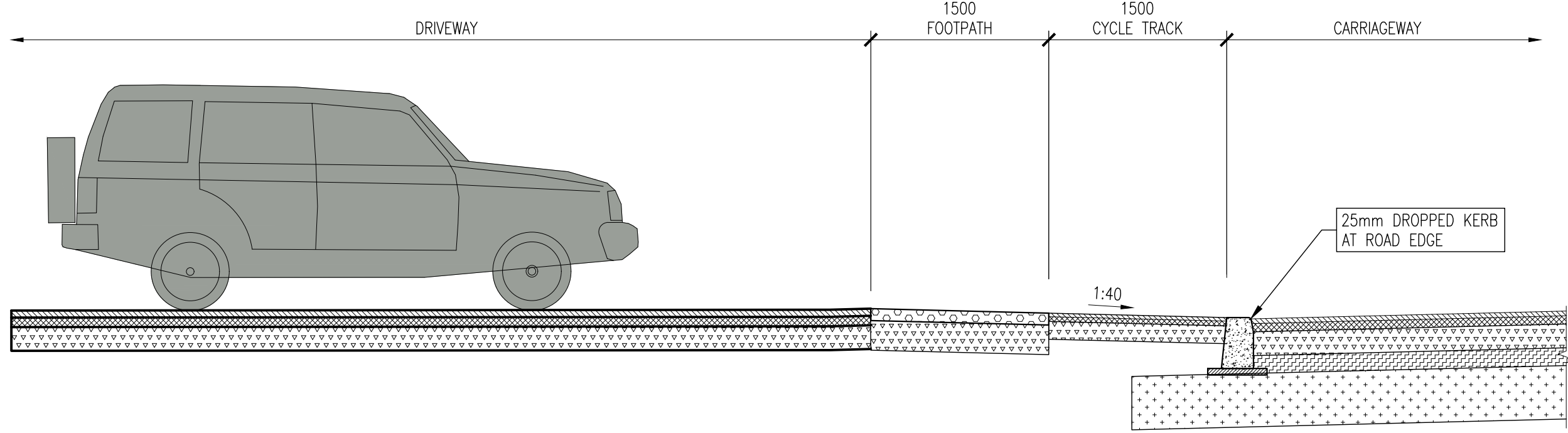
TYPICAL SECTION THROUGH PRIVATE ACCESS SECTION (A-A) SCALE 1:50
