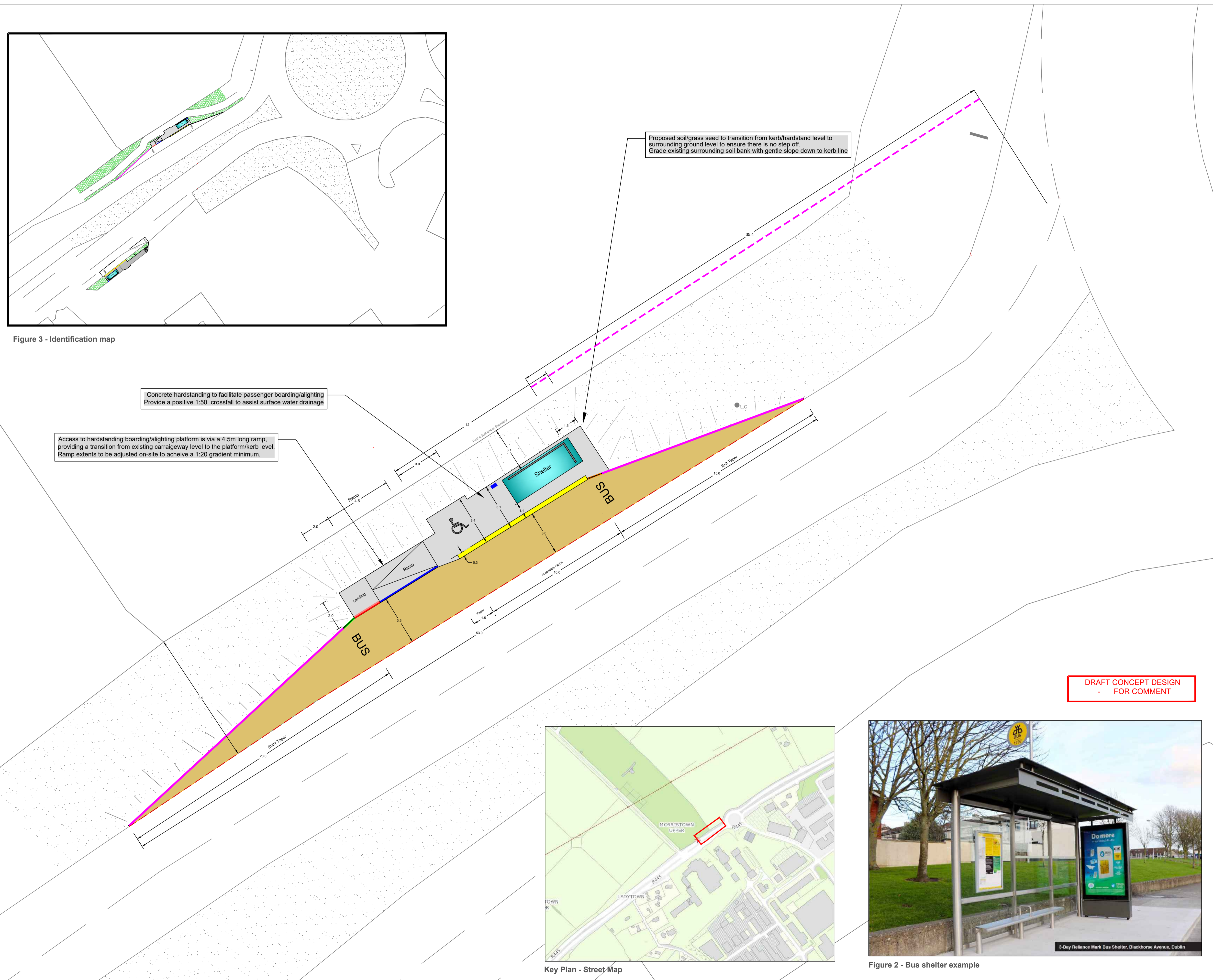
Figure 1 - Layout Plan proposed new Bus Shelter/Boarding platform
