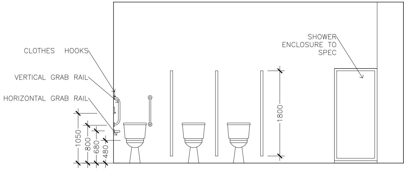
Elevation B Scale 1-50
