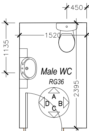
Male WC Plan Scale 1-50
