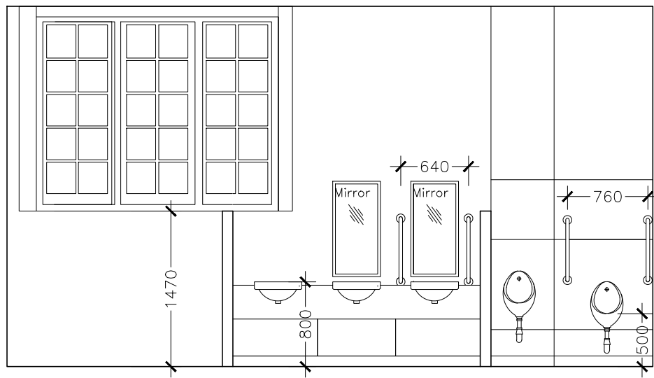
Elevation D Scale 1-50
