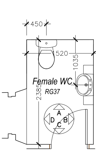
Female WC Plan Scale 1-50
