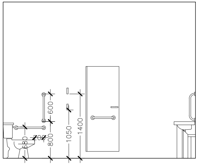
Elevation A Scale 1-50
