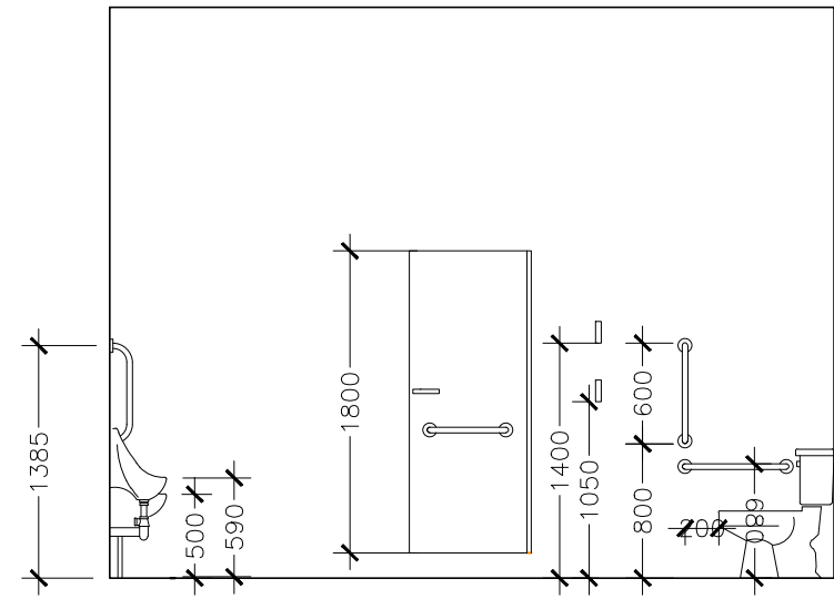
Elevation A Scale 1-50
