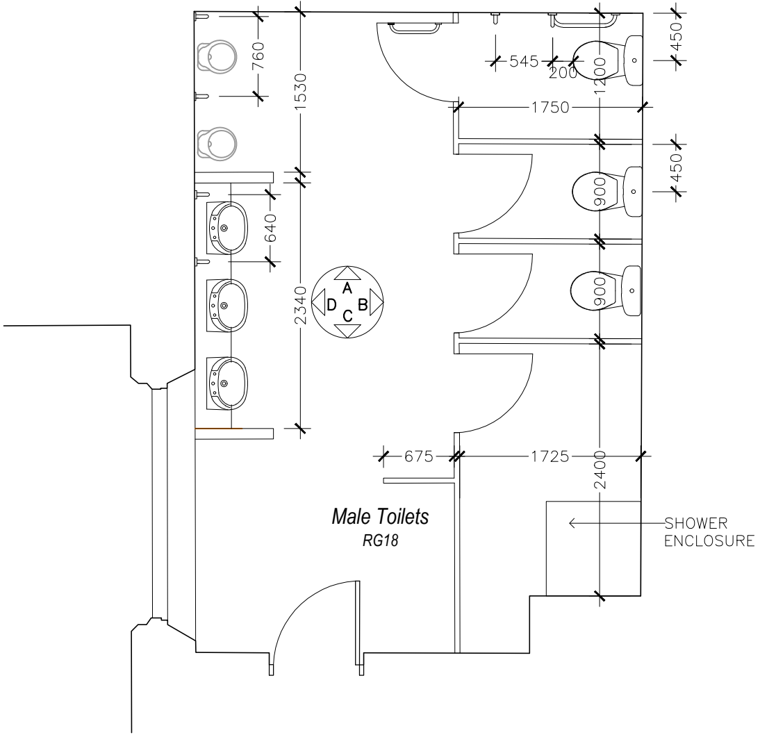
Male Toilets Plan Scale 1-50
