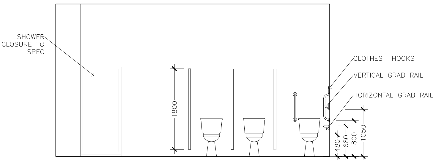
Elevation D Scale 1-50
