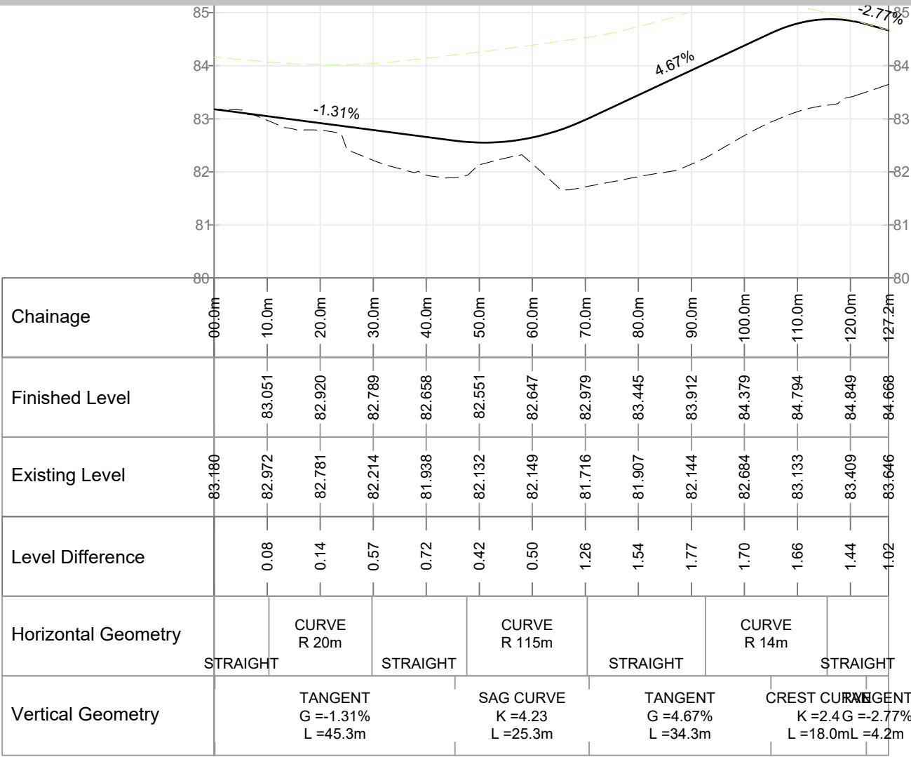
ACCOMMODATION ROAD 01
