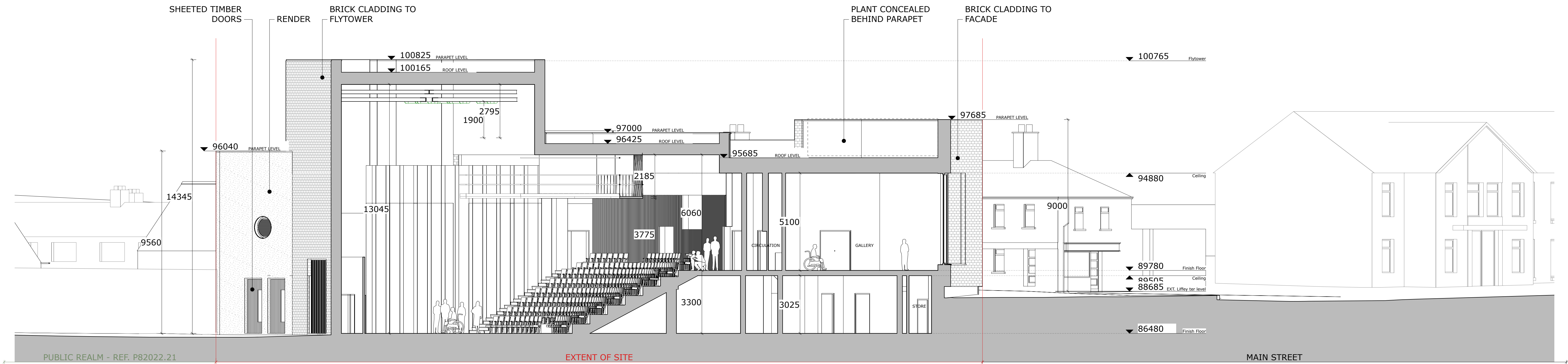
01 PROPOSED SECTION A-A RAC P8 00 201 PART 8 1:100
