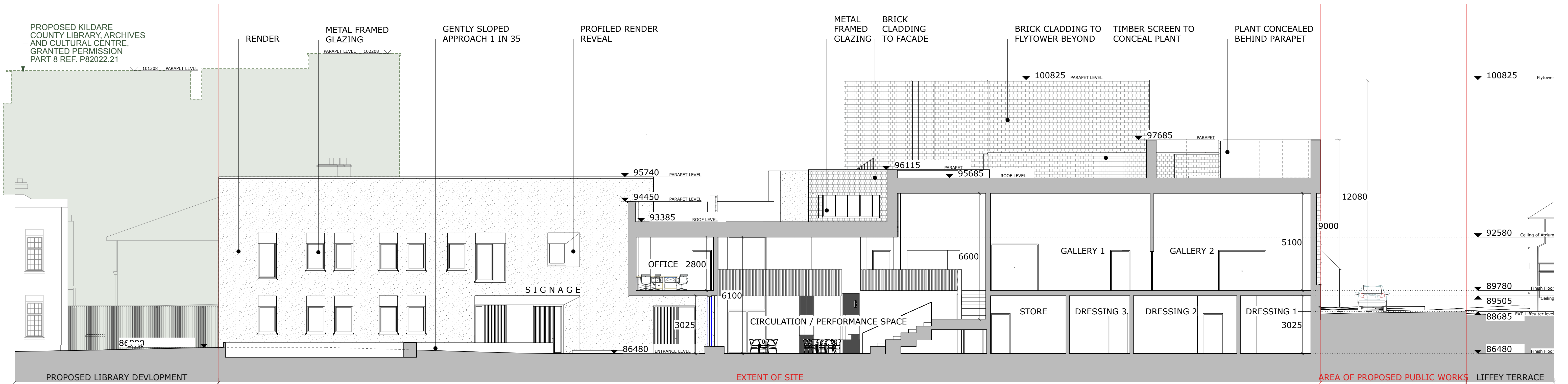
02 PROPOSED SECTION B-B RAC P8 00 201 PART 8 1:100
