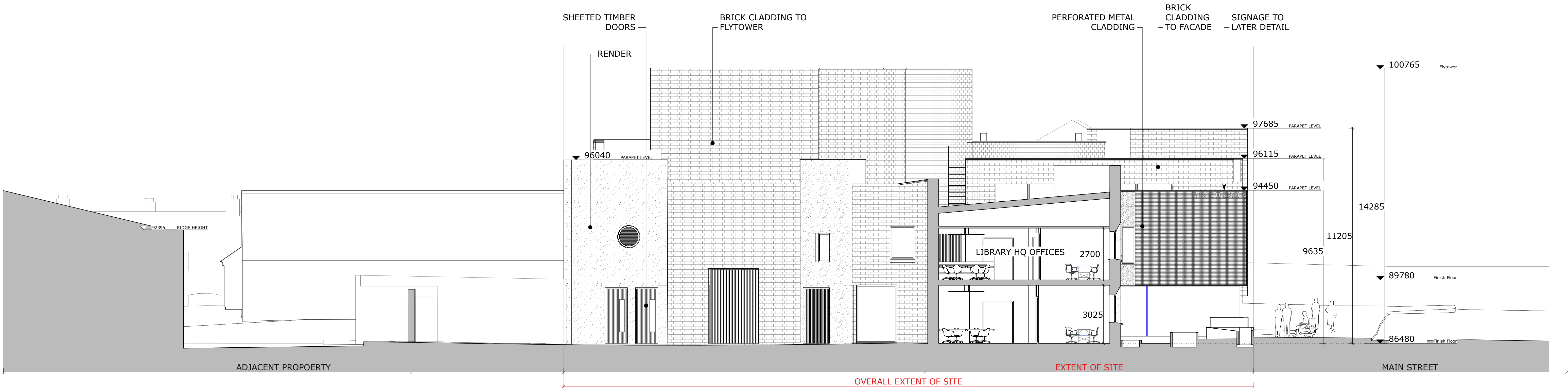
02 P8 00 203 PROPOSED SECTION F-F PART 8 RAC 1:100
