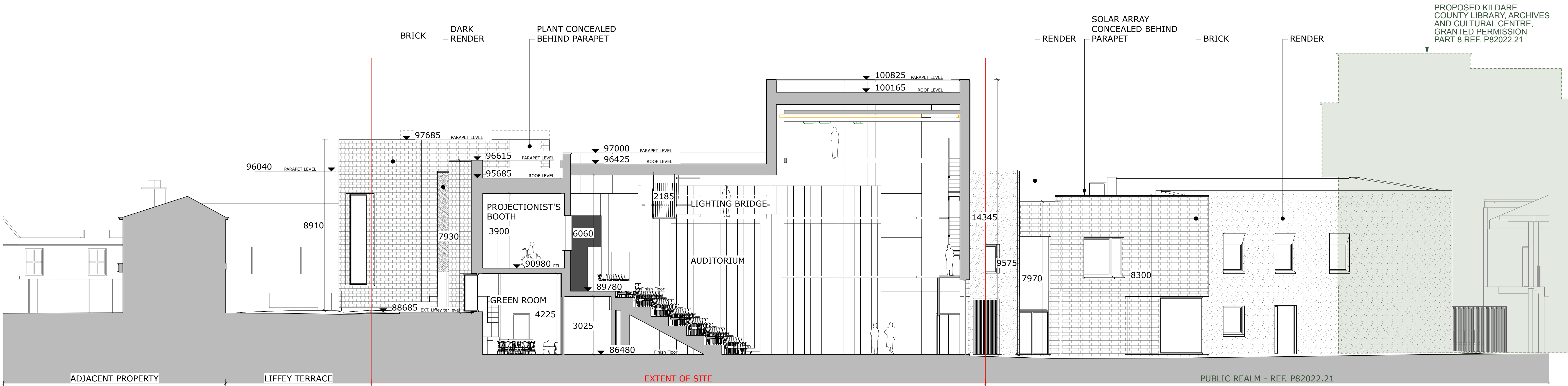
01 P8 00 203 PROPOSED SECTION E-E PART 8 RAC 1:100
