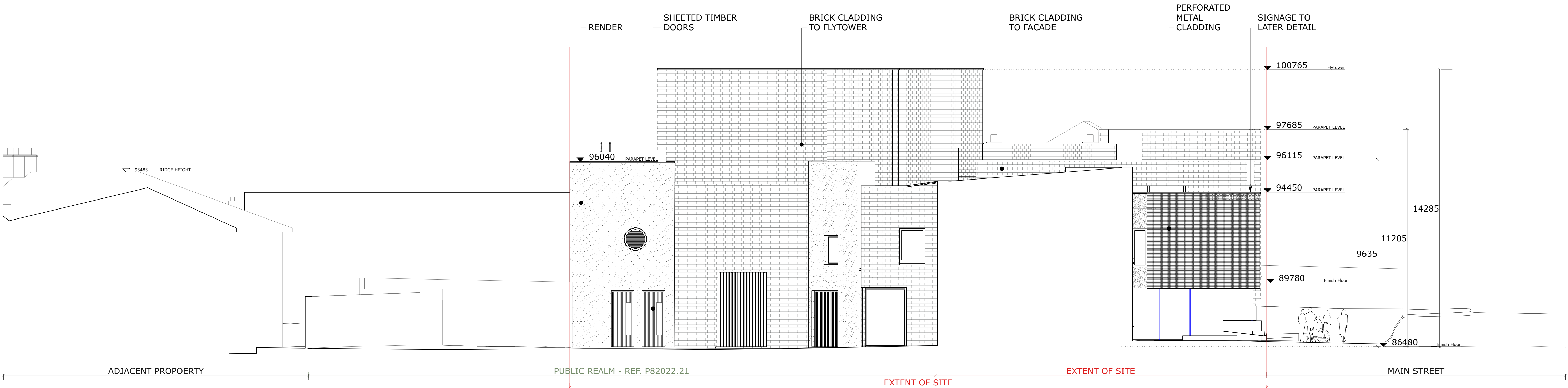
02 PROPOSED EAST FACING ELEVATION RAC P8 00 301 PART 8 1:100
