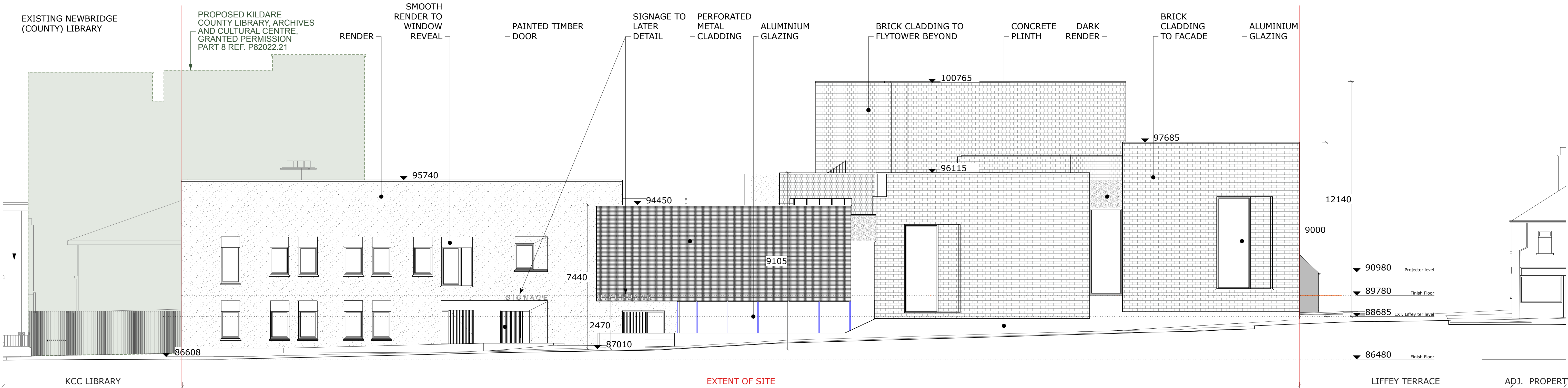
01 PROPOSED NORTH FACING ELEVATION RAC P8 00 301 PART 8 1:100
