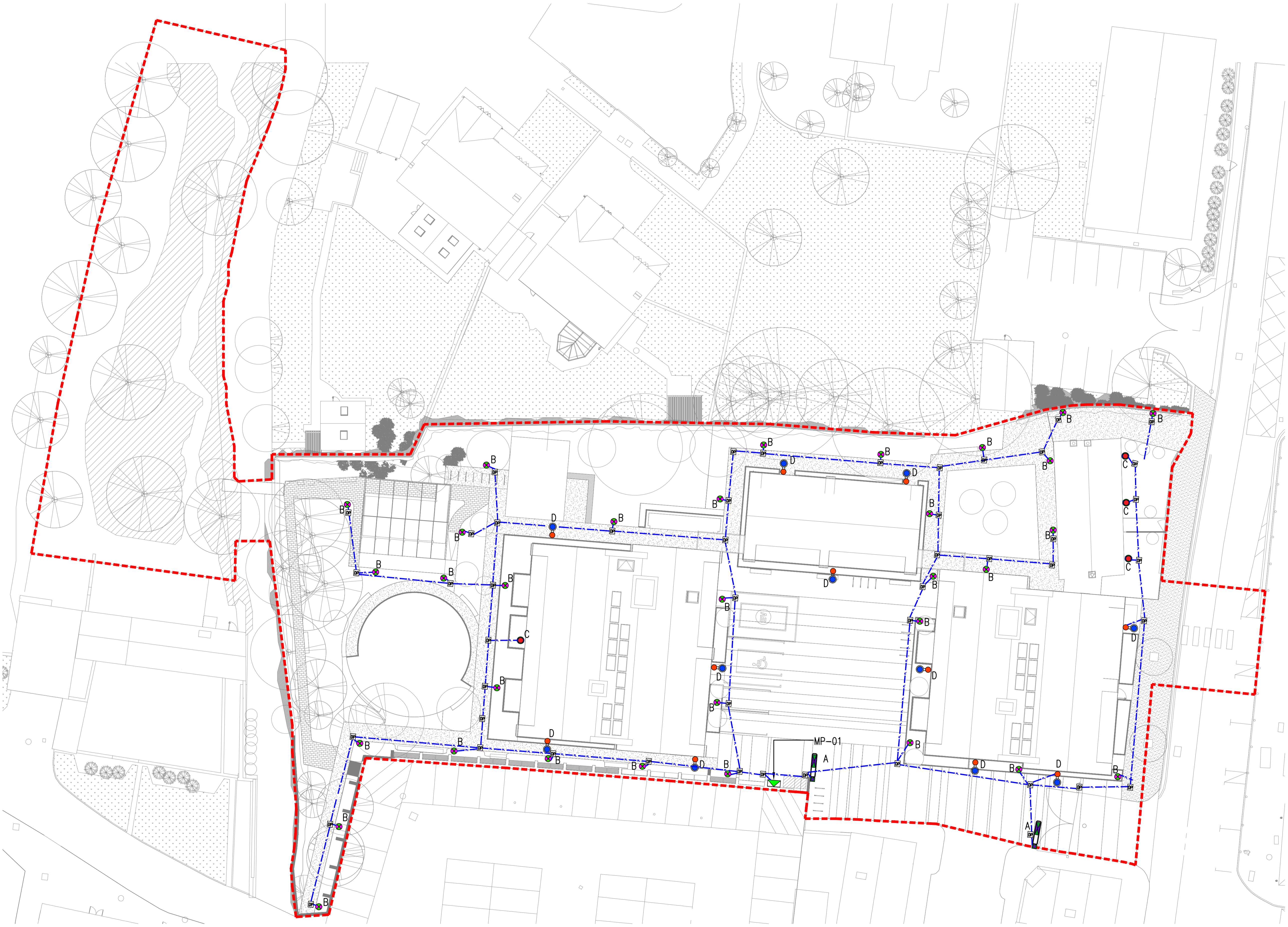
01 SITE LIGHTING AND DUCTING LAYOUT-SITE PLAN 60-S1 SCALE:1:200@A1
